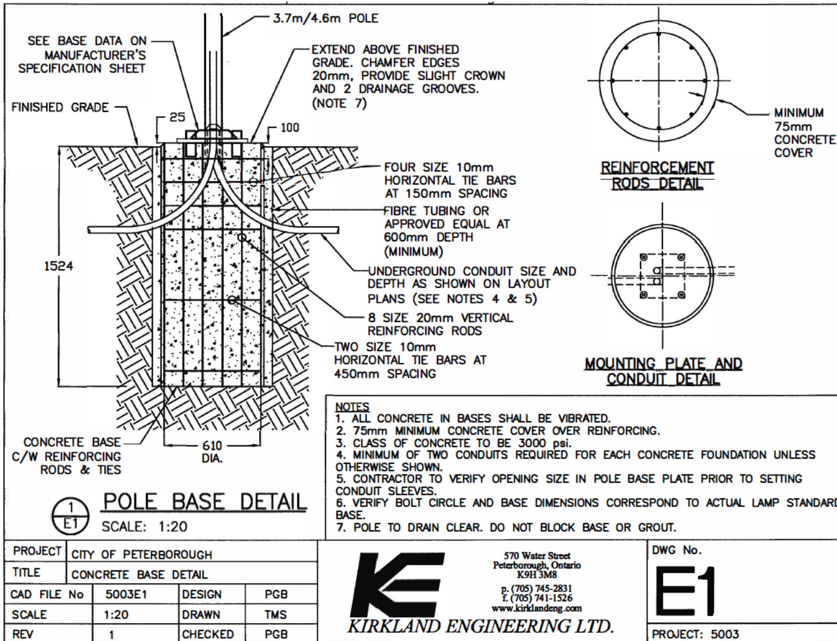
Standard Drawing 6: E1-Pole Base Detail
